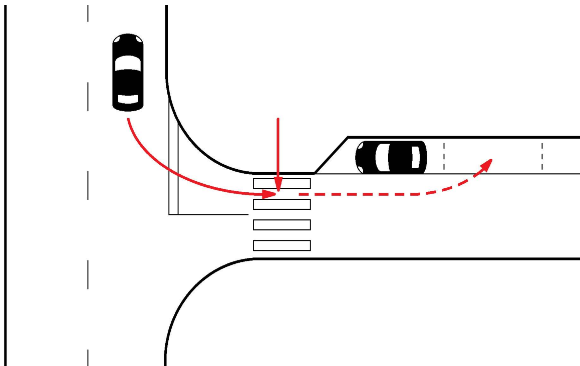
Fig. (1). Vehicle reversing into a perpendicular street to reach a parking space.
