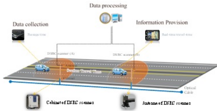
Fig. (1). Schematic of the DSRC traffic information system.
