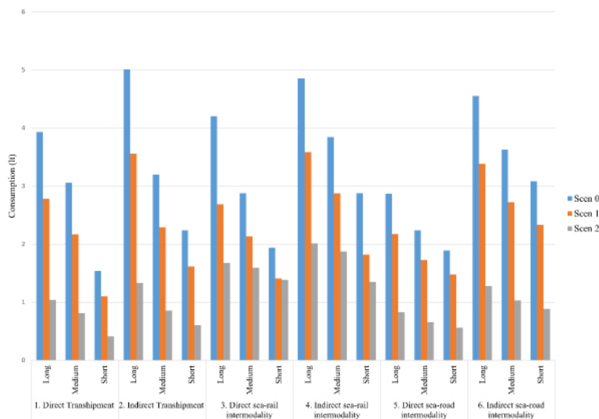
Fig. (7). Energy consumption in Scenario 0, 1 e 2.
